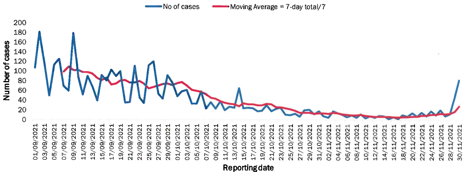
Figure 1: The 7 days moving average line chart for confirmed COVID-19 cases, 30 November 2021
